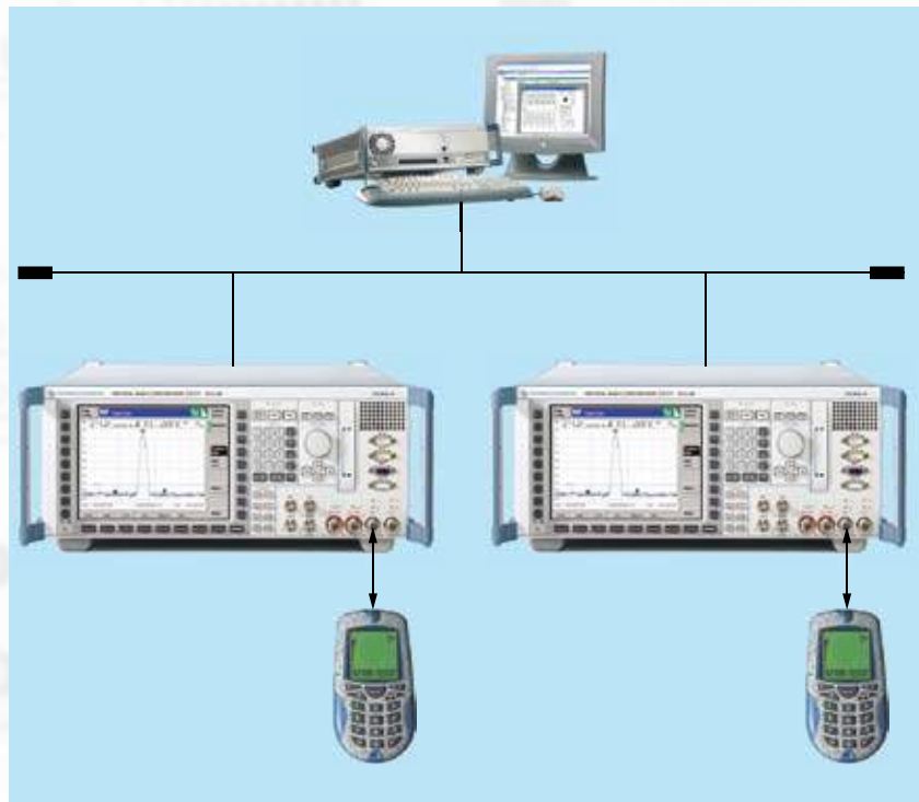
A test setup for an end-to-end test between two mobile phones for testing for problem-free MMS exchange between mobile phones from different manufacturers, for example.
