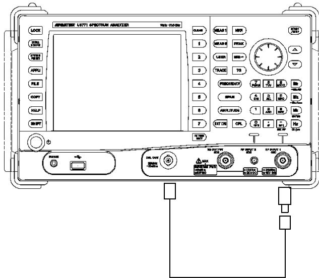
Figure 3-7 Connecting the CAL Signal
