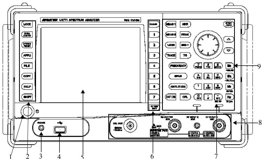
Figure 4-1 Front Panel
