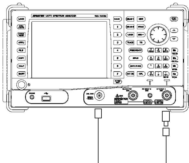
Figure 4-16 Connecting the CAL Signal
