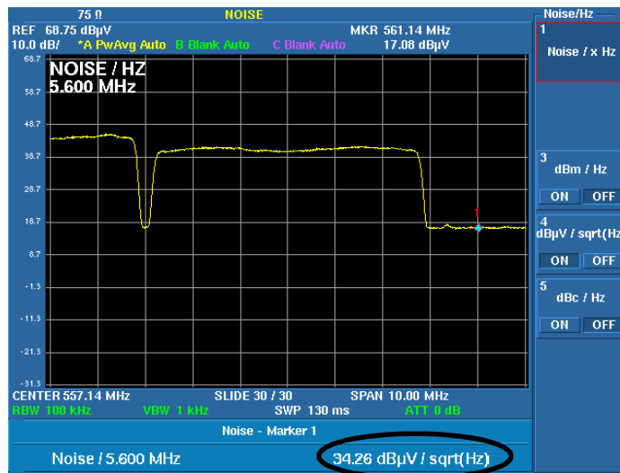
Figure 4-22 Measurement Display for Noise Power Converted into 5.6 MHz Bandwidth
