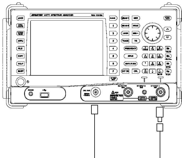
Figure 4-9 Connecting the CAL Signal (RF INPUT1 connector)
